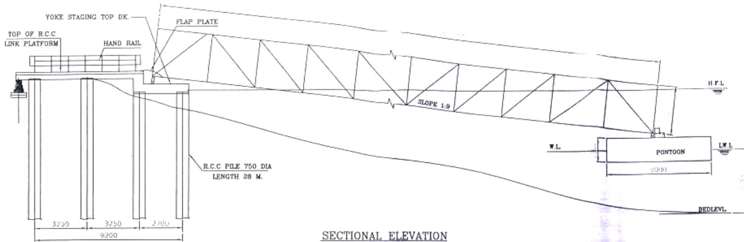
SECTIONAL ELEVATION
