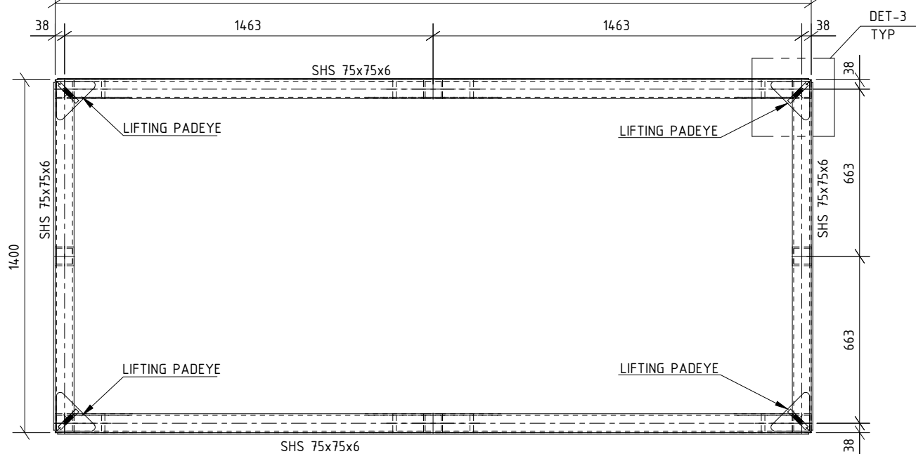
PLAN VIEW (SCALE 1:20)
