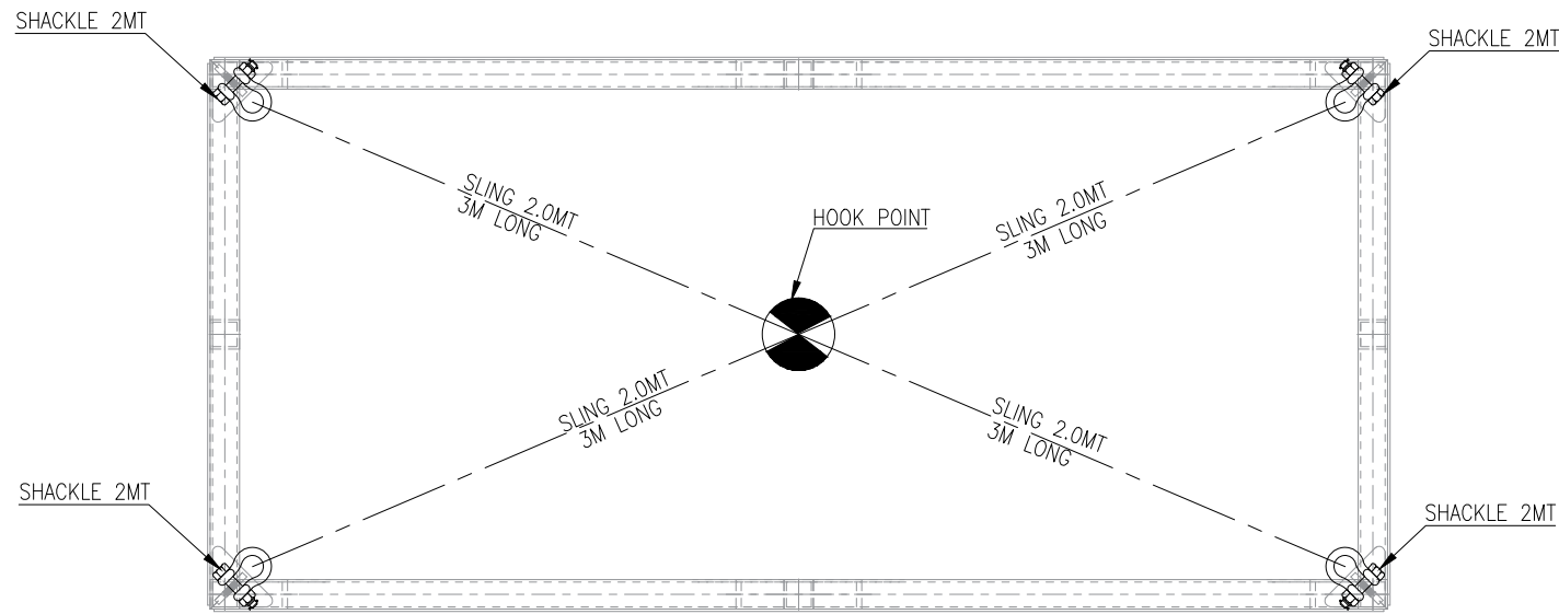
MATERIAL LIFTING BASKET (3.0 MT S.W.L.) UPPER PLAN VIEW
