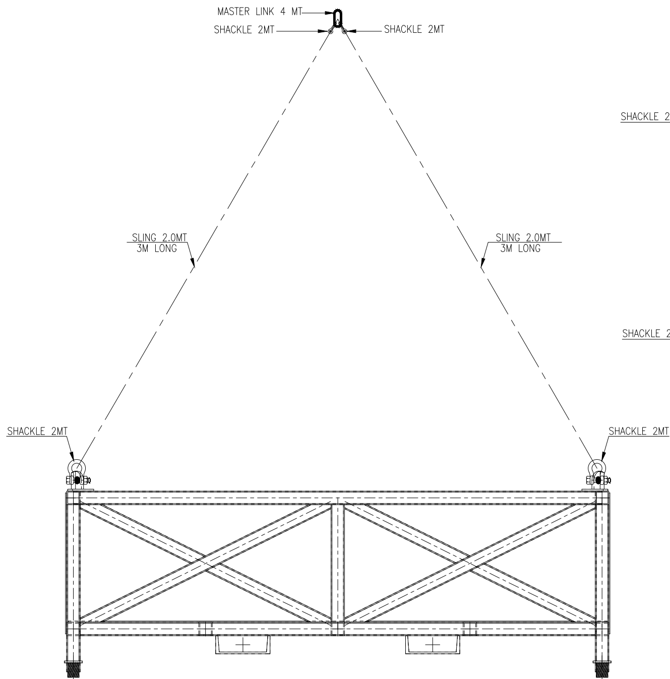
MATERIAL LIFTING BASKET (3.0 MT S.W.L.) FRONT EL.VIEW
