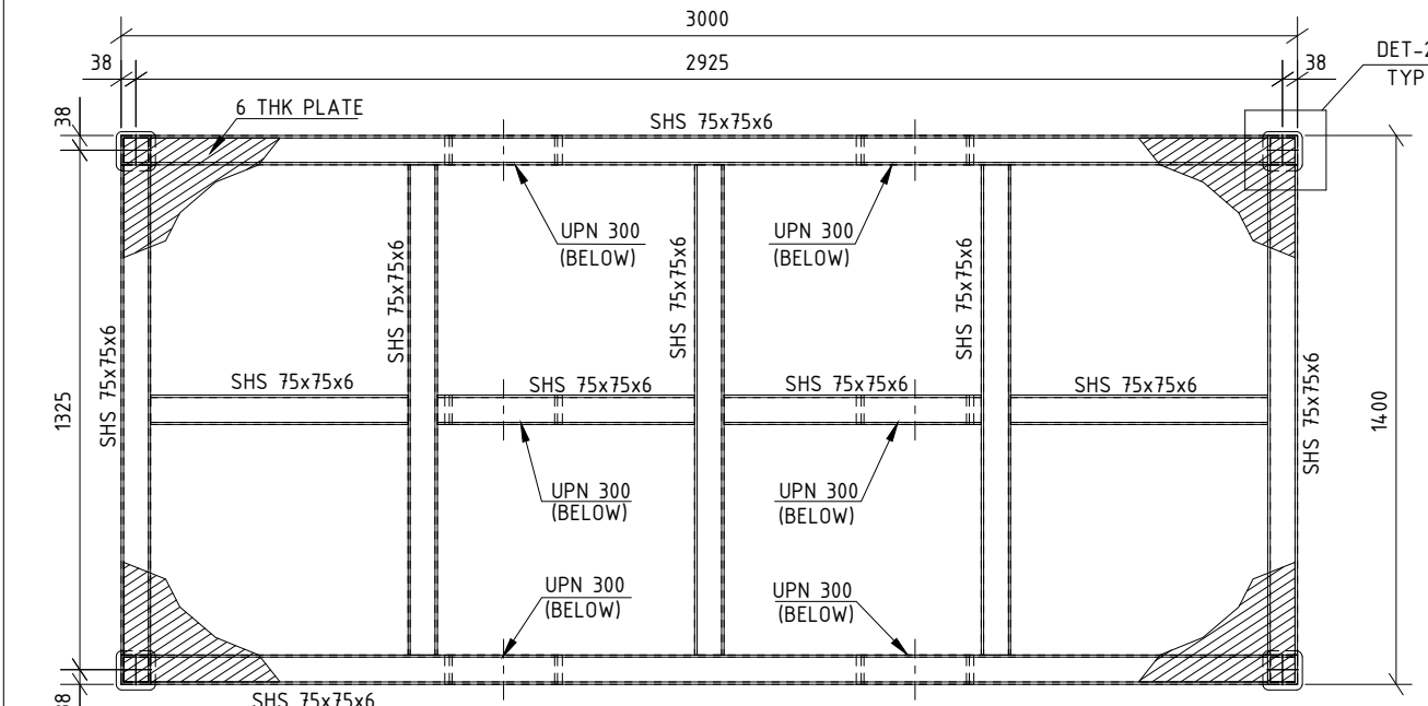
BOTTOM VIEW (SCALE 1:20)
