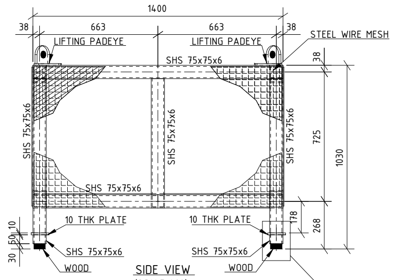
SEC A - A (SCALE 1:20)
